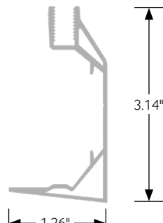
Fixed Perimeter Extrusion (optional)
