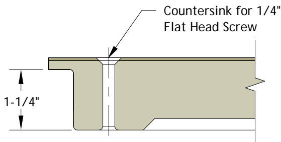
BARE CORNER-LOCK PANEL
