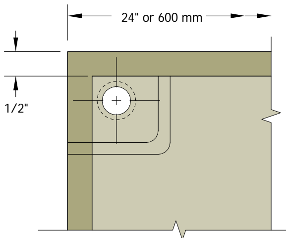
PARTIAL BOTTOM VIEW
