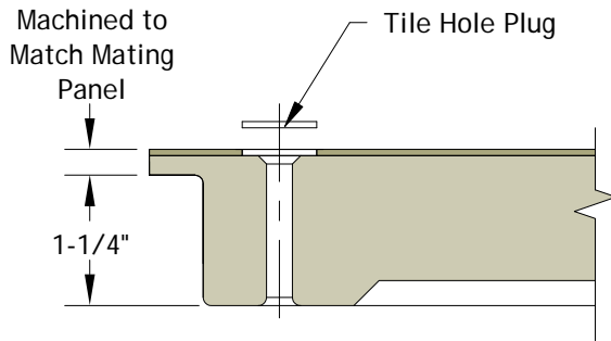
TILE COVERED CORNER-LOCK PANEL
