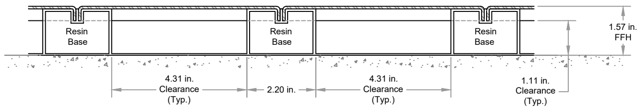
Q2C-40 (1.5" FFH) UNDERFLOOR CLEARANCE
