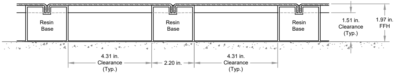
Q2C-50 (2" FFH) UNDERFLOOR CLEARANCE
