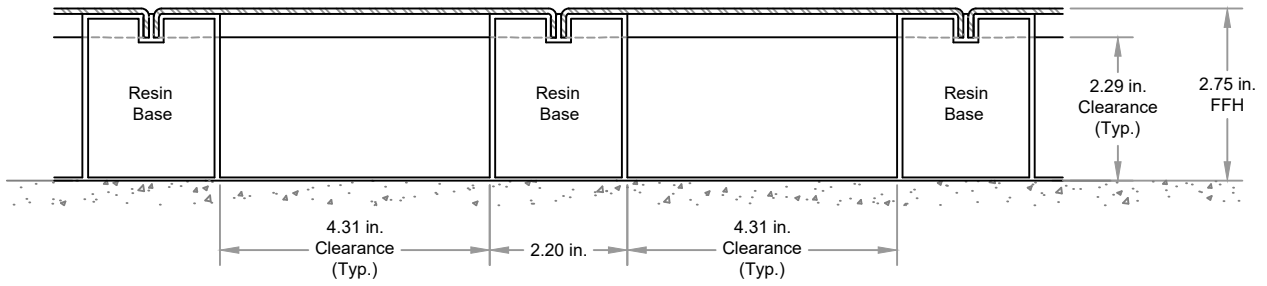
Q2C-70 (2.75" FFH) UNDERFLOOR CLEARANCE
