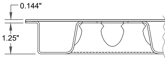
PARTIAL SIDE VIEW
