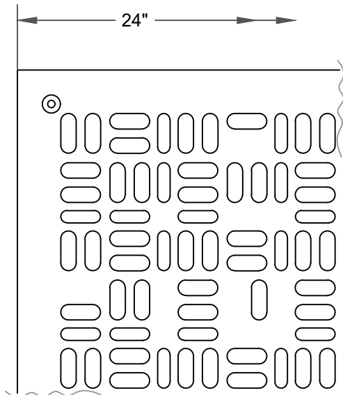
PARTIAL TOP VIEW (ADA Compliant)
