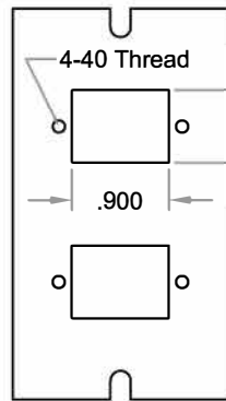
DP012 For (2) Modular L-COM Couplers
