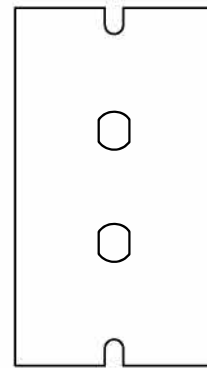
DP008 For (2) "ST" Style Connectors
