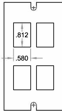
DP007A For (4) Modular Jack Couplers
