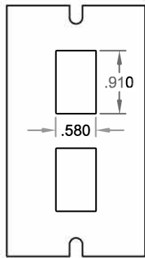
DP006 For (2) Modular Jack Couplers
