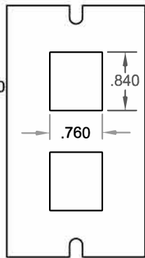
DP011 For (2) Modular Jack Couplers
