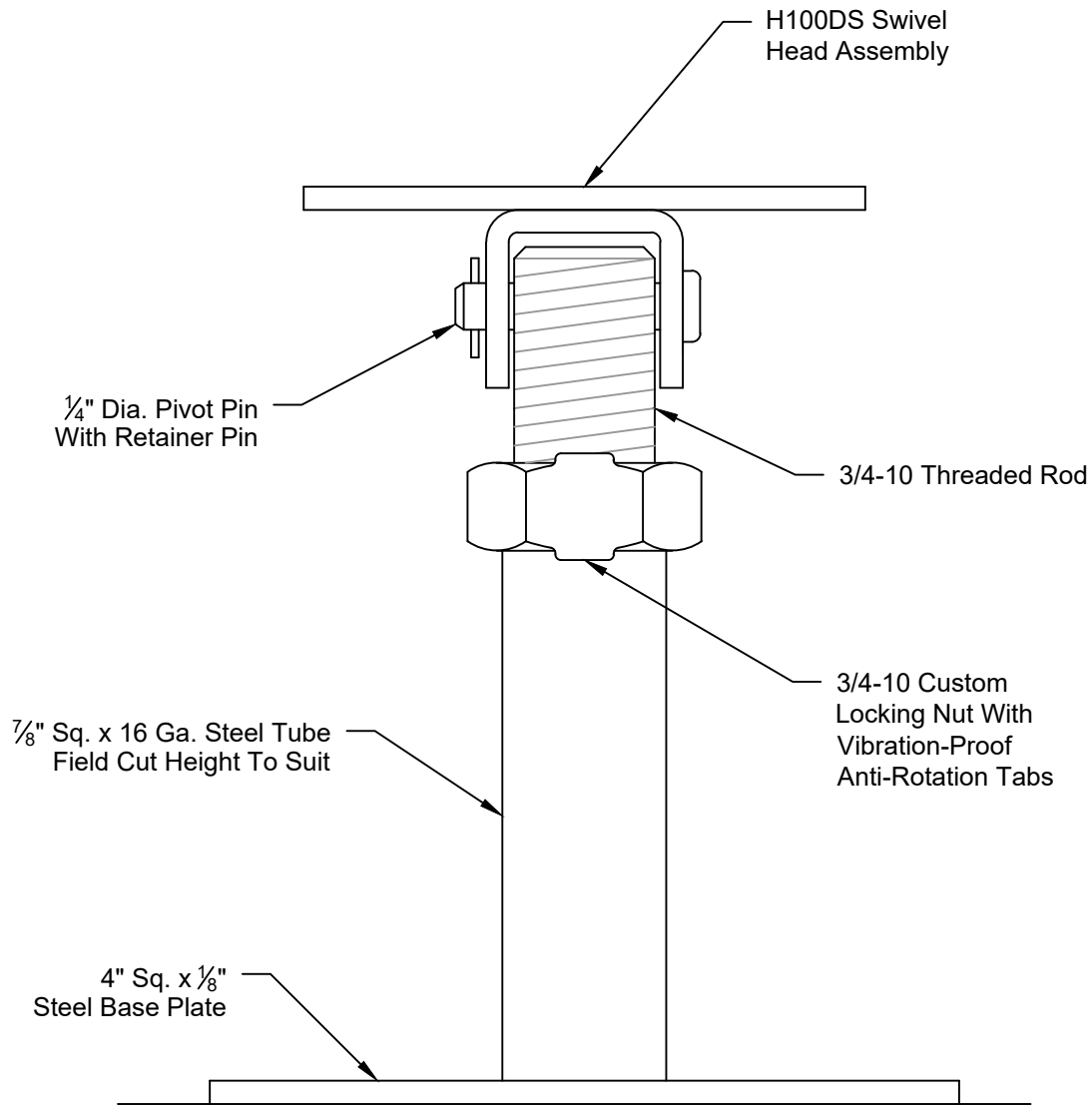
SIDE ELEVATION DETAIL
