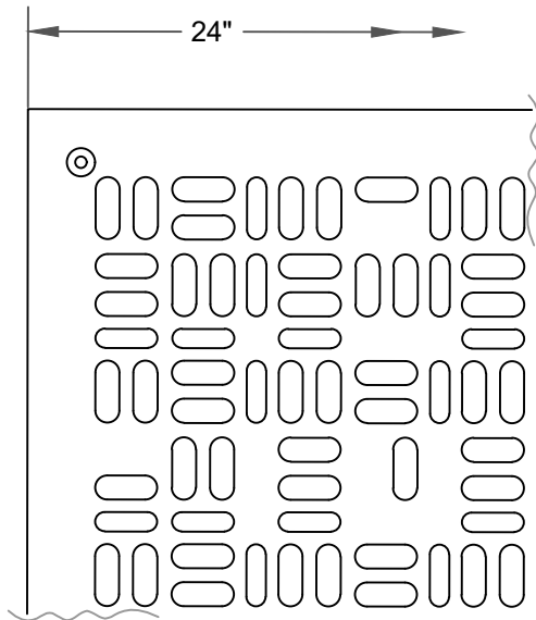
PARTIAL TOP VIEW (ADA Compliant)
