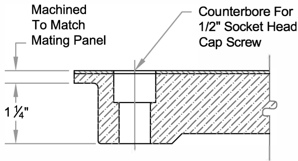
TILE COVERED CORNER BOLTED PANEL
