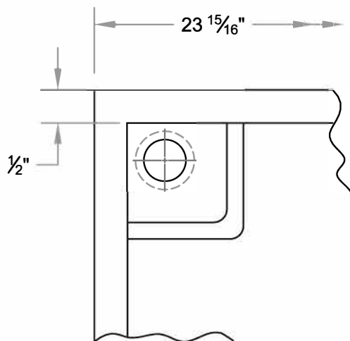
PARTIAL BOTTOM VIEW
