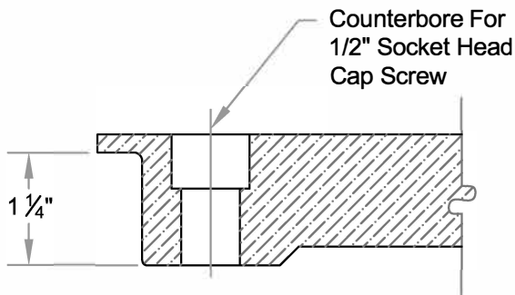
BARE SURFACE CORNER BOLTED PANEL
