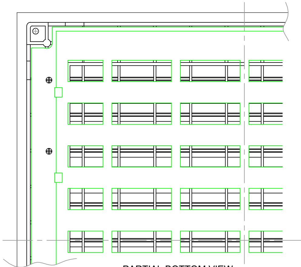
PARTIAL BOTTOM VIEW (Shown With Damper 100% Open)
