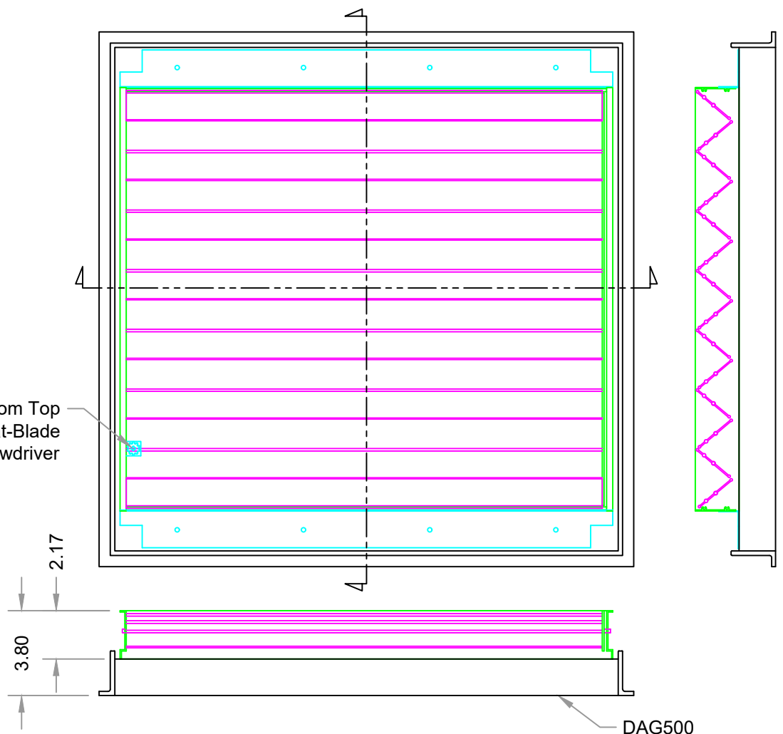
DAG500 DIRECTIONAL AIR FLOW GRATE 24" or 600mm Size
